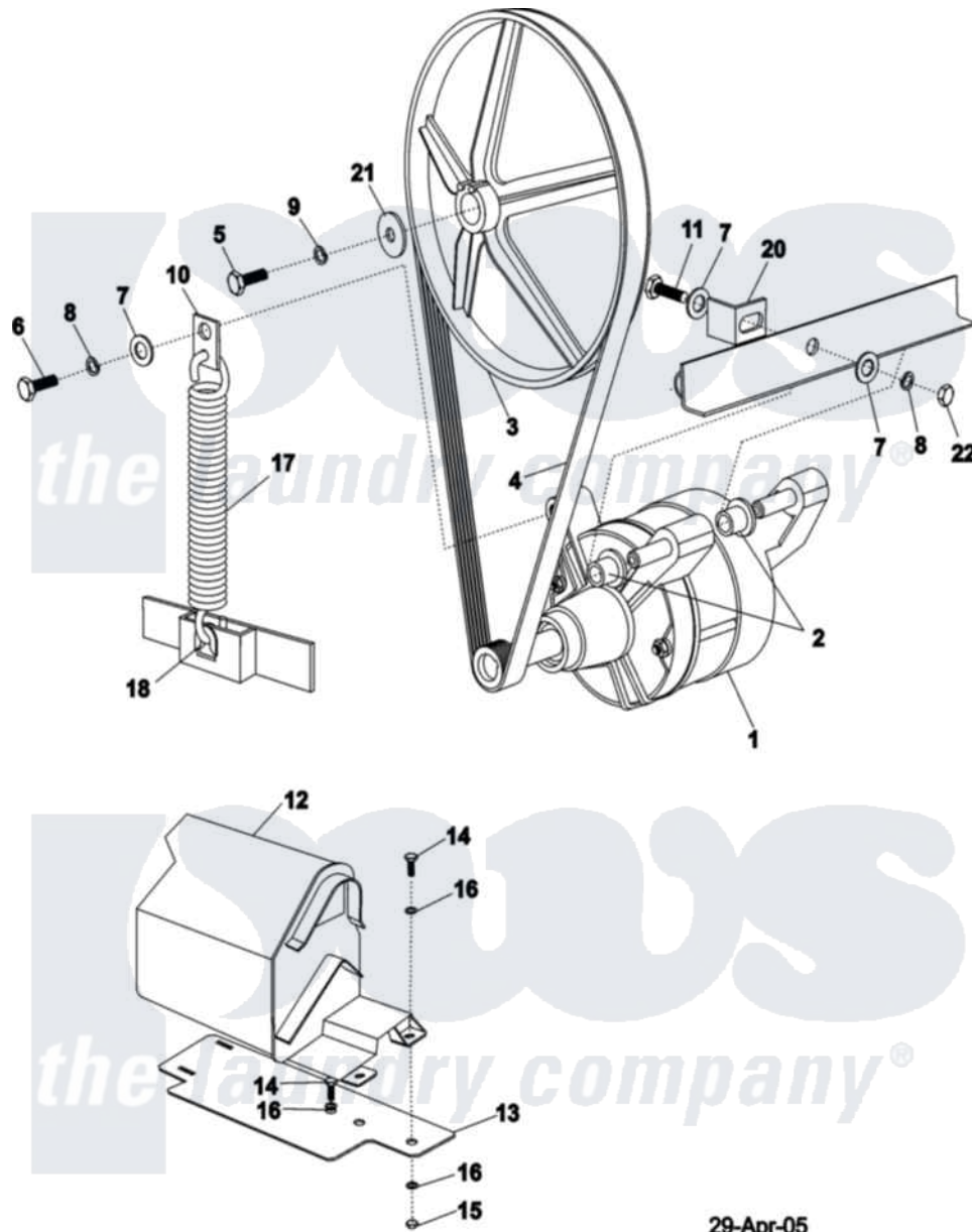
Maytag Commercial Maytag MFR18PDCWS Washer Parts Parts Diagram 10 - MOTOR AND DRIVE ASY Click on the part number to view part
