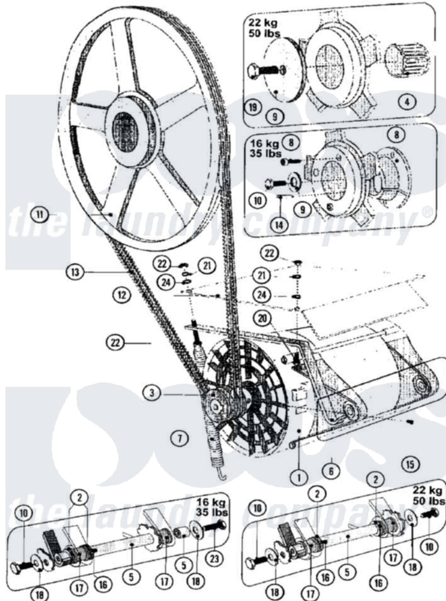
Maytag Commercial Maytag MFR35MNATS Washer Parts Parts Diagram 24 - MOTOR & BASKET PULLEY (SERIES 11)
