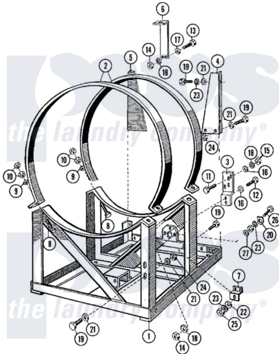
Maytag Commercial Maytag MFR35PCATS Washer Parts Parts Diagram 12 - BASE FRAME Click on the part number to view part
