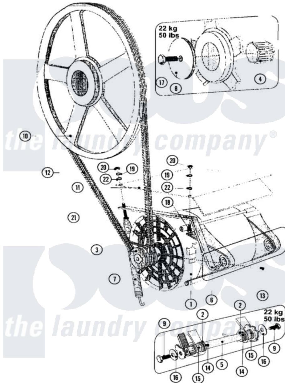
Maytag Commercial Maytag MFR50MCAVS Washer Parts Parts Diagram 23 - MOTOR & BASKET PULLEY (SERIES 11)
