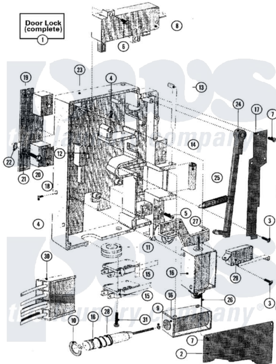
Maytag Commercial Maytag MFR50PCATS Washer Parts Parts Diagram 19 - DOOR LOCK ASSEMBLY (SERIES 11)
