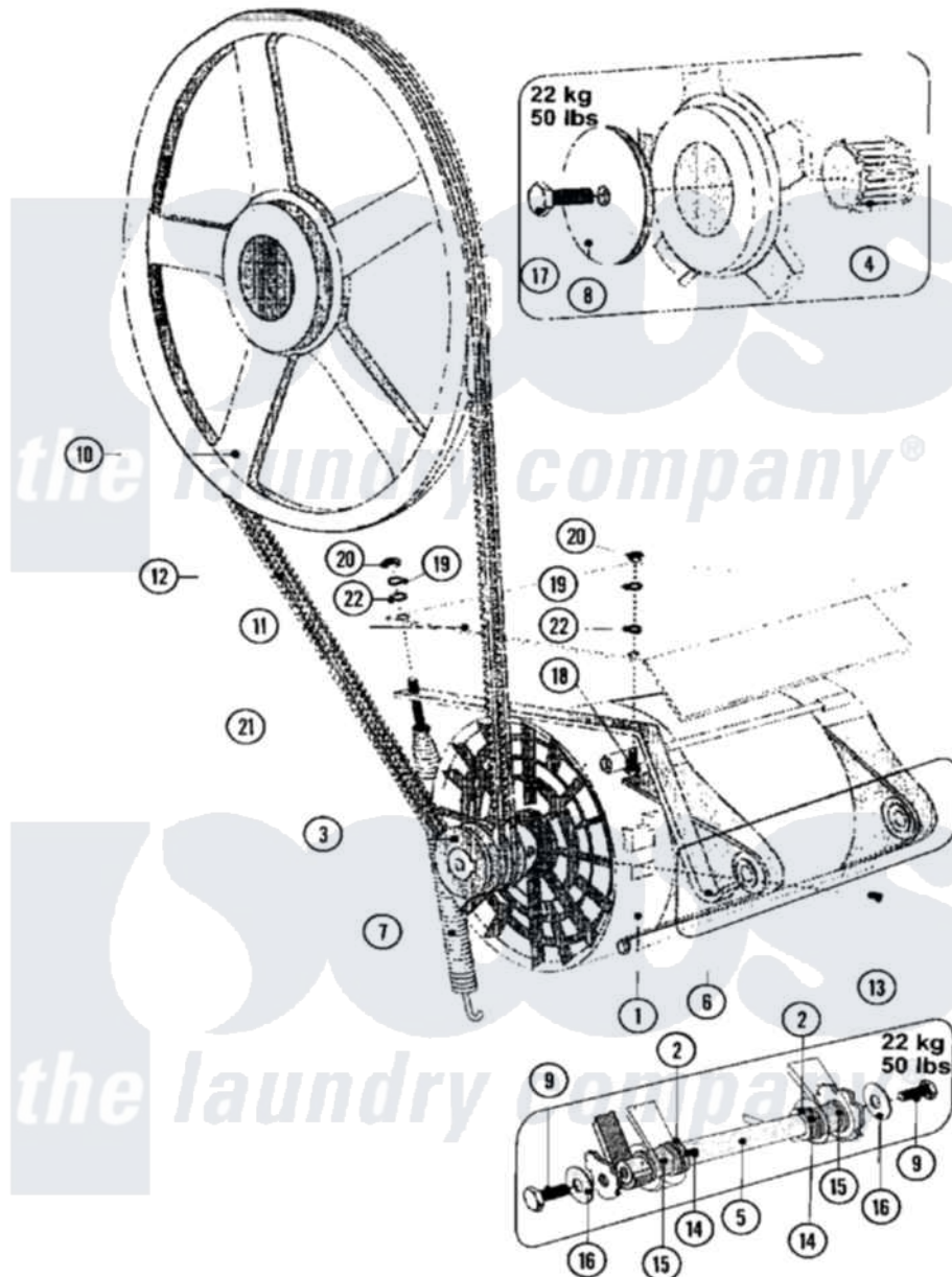
Maytag Commercial Maytag MFR50PCAVS Washer Parts Parts Diagram 22 - MOTOR & BASKET PULLEY (SERIES 11)
