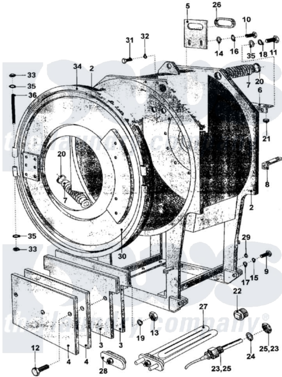
Maytag Commercial Maytag MFS100PAVS Washer Parts Parts Diagram 04 - TUB Click on the part number to view part
