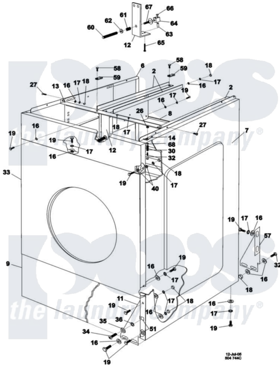
Maytag Commercial Maytag MFS25PNFTS Washer Parts Parts Diagram 02 - CABINET Click on the part number to view part
