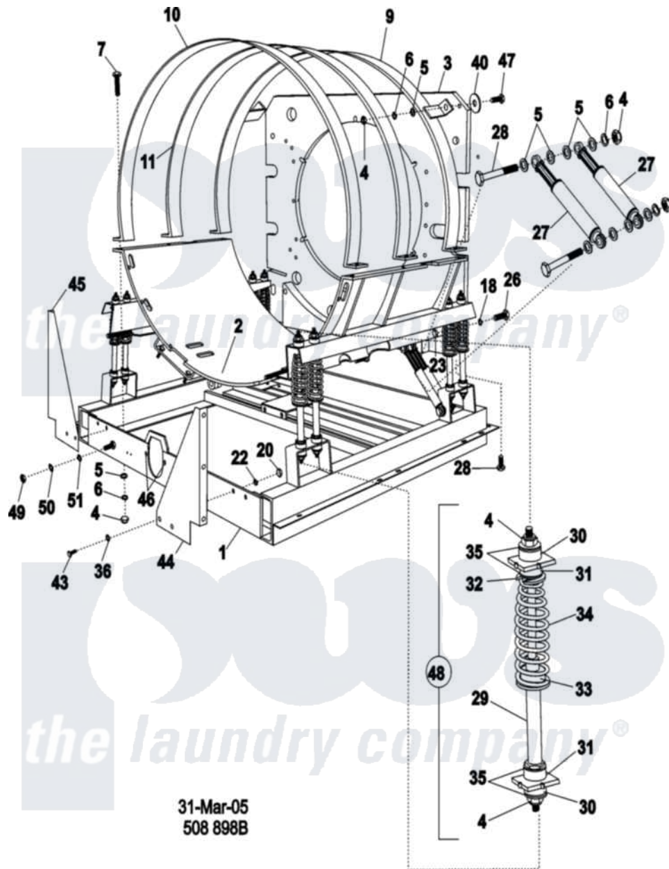
Maytag Commercial Maytag MFS35PNFTS Washer Parts Parts Diagram 01 - FRAME AND TUB SUPPORT Click on the part number to view part
