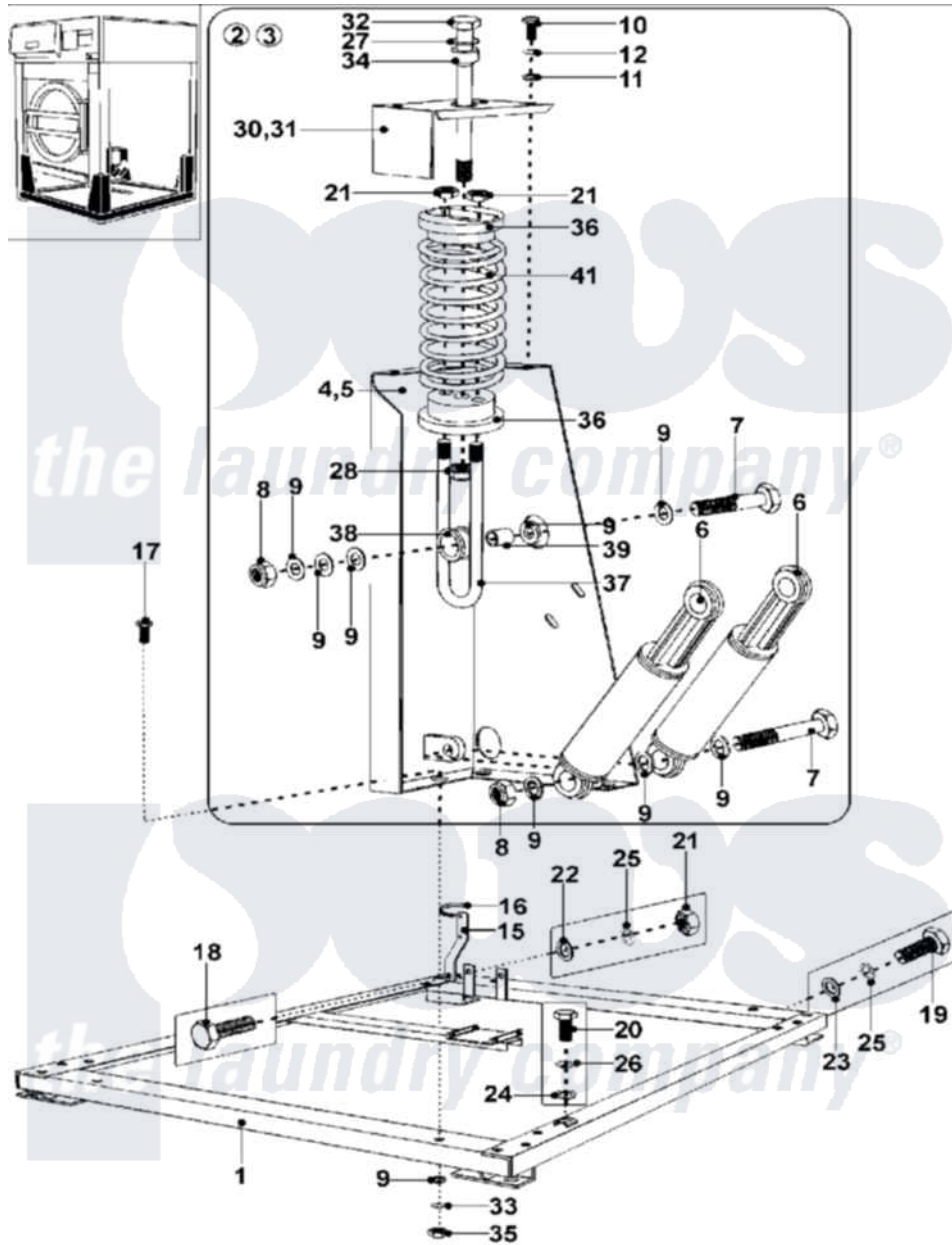
Maytag Commercial Maytag MFS50PNDVS Washer Parts Parts Diagram 01 - BASE Click on the part number to view part
