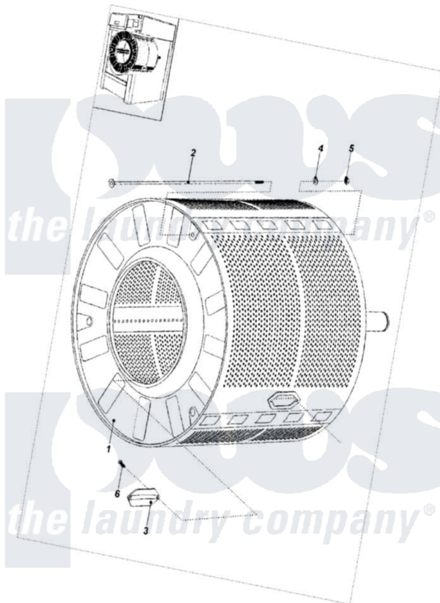
Maytag Commercial Maytag MFS50PNDVS Washer Parts Parts Diagram 04 - INNER TUB Click on the part number to view part
