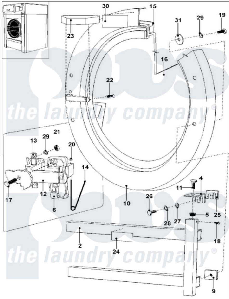
Maytag Commercial Maytag MFS50PNDVS Washer Parts Parts Diagram 09 - DOOR Click on the part number to view part
