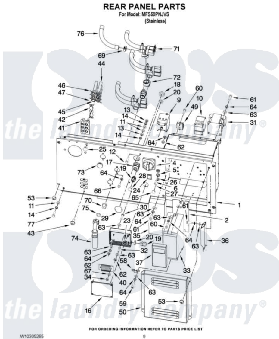
Maytag Commercial Maytag MFS50PNJVS Washer Parts Parts Diagram 07 - REAR PANEL PARTS Click on the part number to view part
