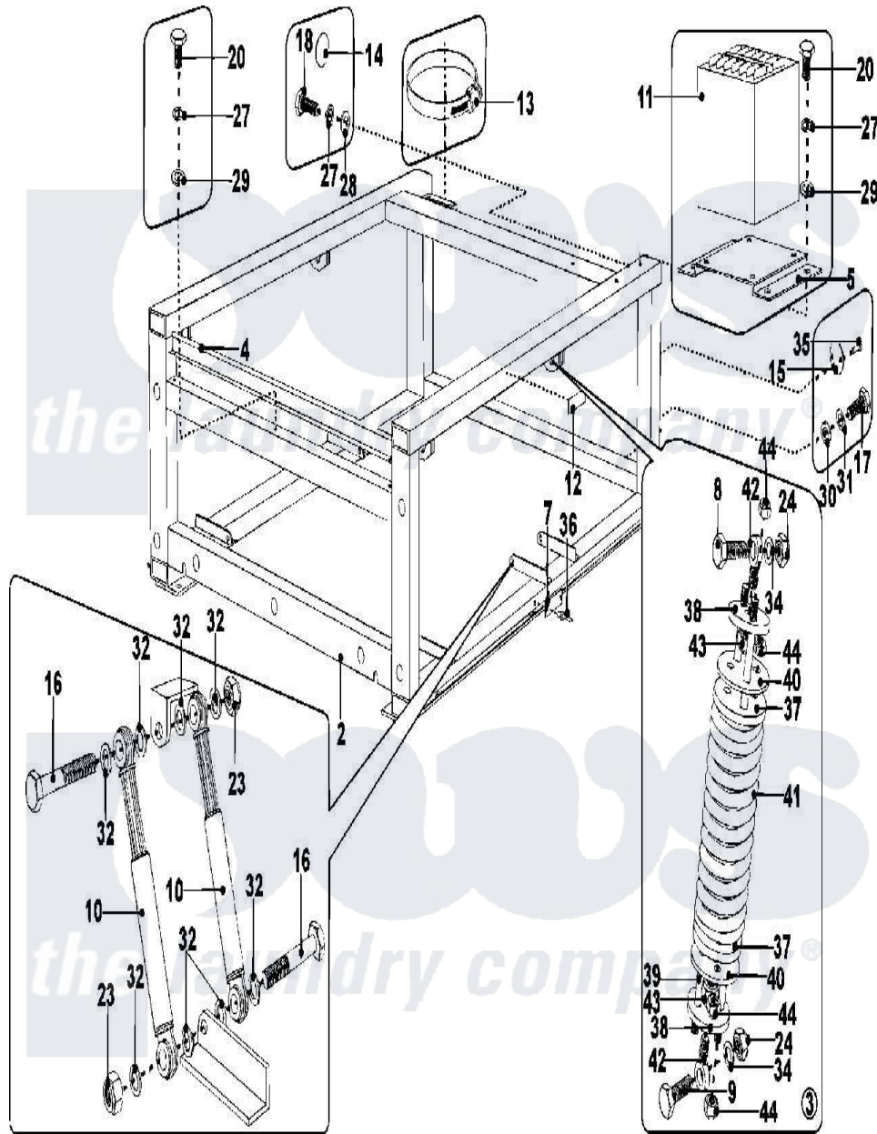
Maytag Commercial Maytag MFS80PNDVS Washer Parts Parts Diagram 01 - BASE Click on the part number to view part
