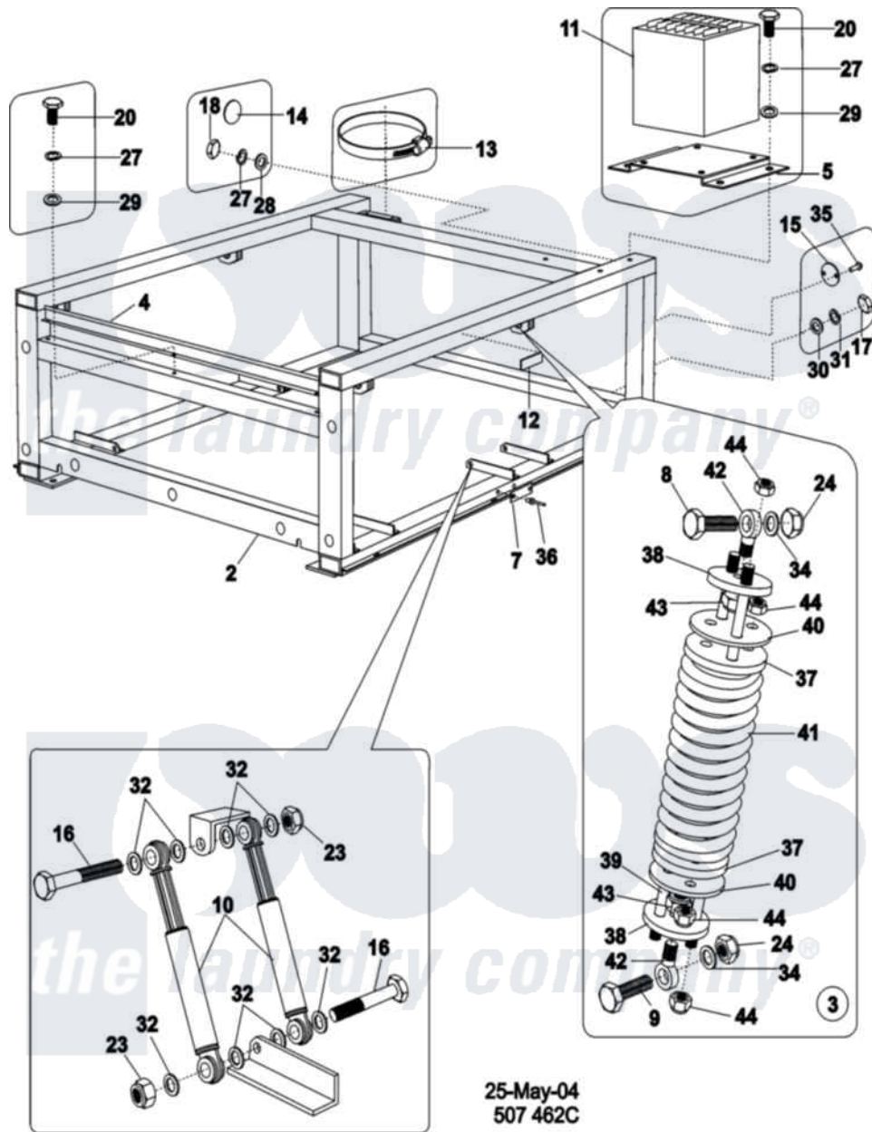
Maytag Commercial Maytag MFS80PNFVS Washer Parts Parts Diagram 01 - FRAME Click on the part number to view part
