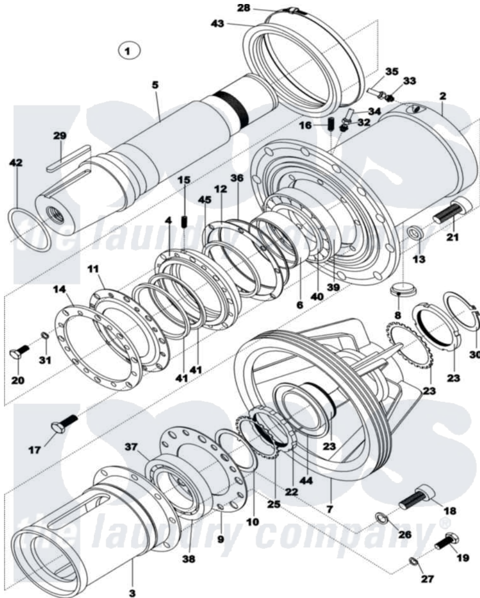
Maytag Commercial Maytag MFS80PNFVS Washer Parts Parts Diagram 06 - TRUNNION 80LB Click on the part number to view part
