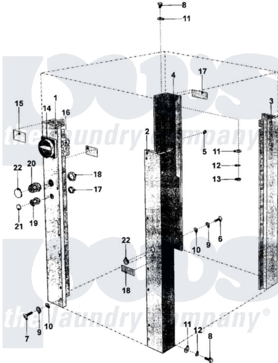
Maytag Commercial Maytag MFS90PNAVS Washer Parts Parts Diagram 02 - CABINET Click on the part number to view part
