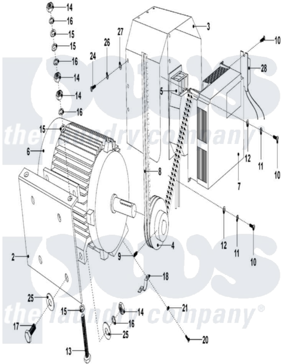
Maytag Commercial Maytag MFX50NNATS Washer Parts Parts Diagram 08 - MOTOR AND PULLEY Click on the part number to view part
