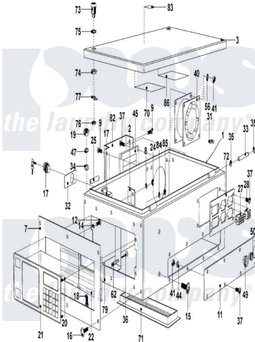
Maytag Commercial Maytag MFX50NNATS Washer Parts Parts Diagram 10 - CONTROL PANEL Click on the part number to view part
