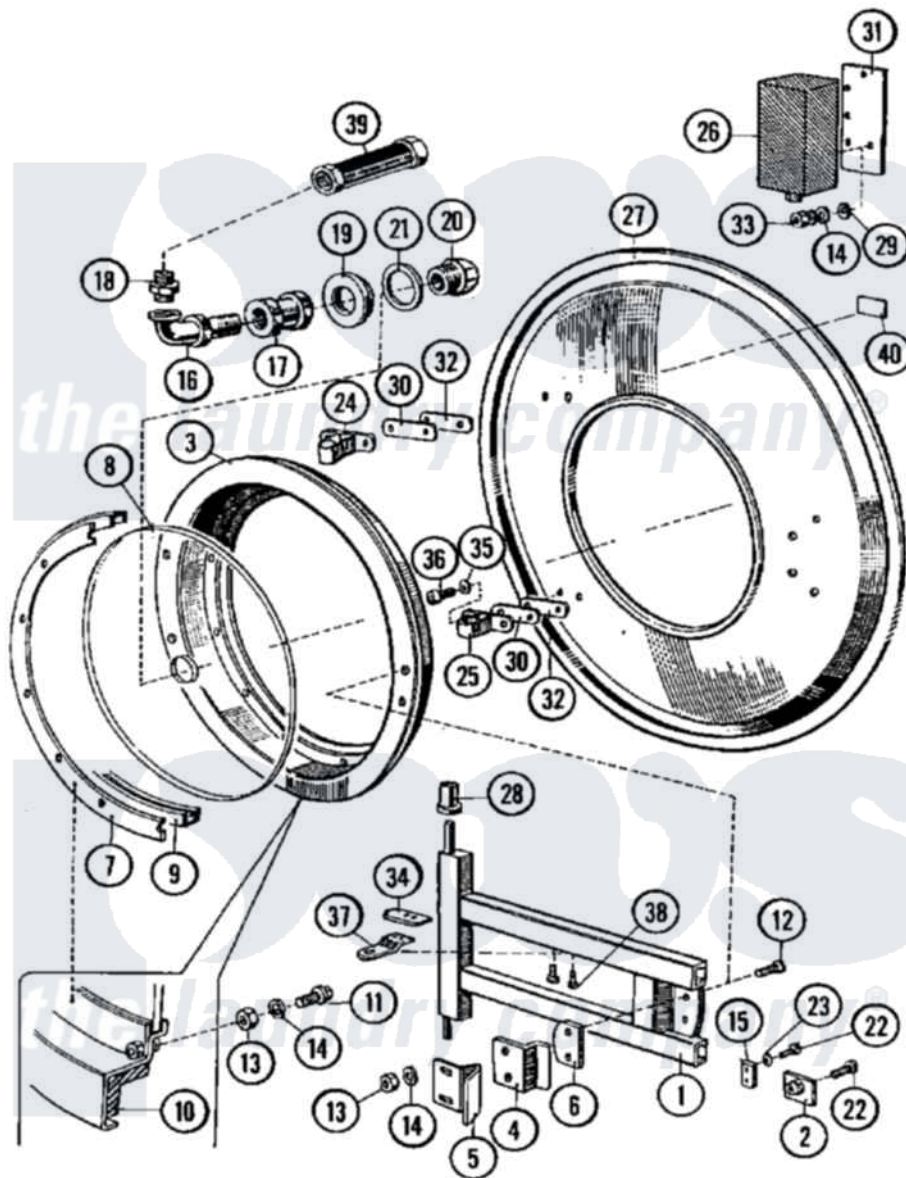
Maytag Commercial Maytag MFX75PNAVS Washer Parts Parts Diagram 07 - DOOR Click on the part number to view part
