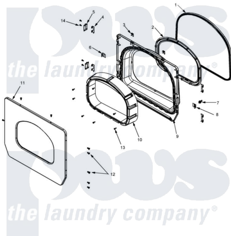
Maytag Commercial Maytag MLE23PDFZW Dryer Parts Parts Diagram 05 - DOOR Click on the part number to view part
