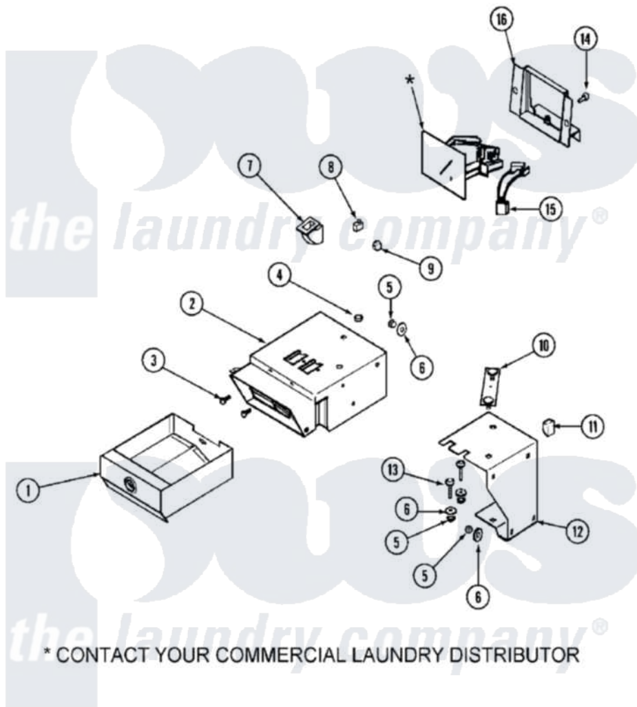
Maytag Commercial Maytag MLG19PDBGW Dryer Parts Parts Diagram 02 - CONTROL CENTER (DRYER) Click on the part number to view part
