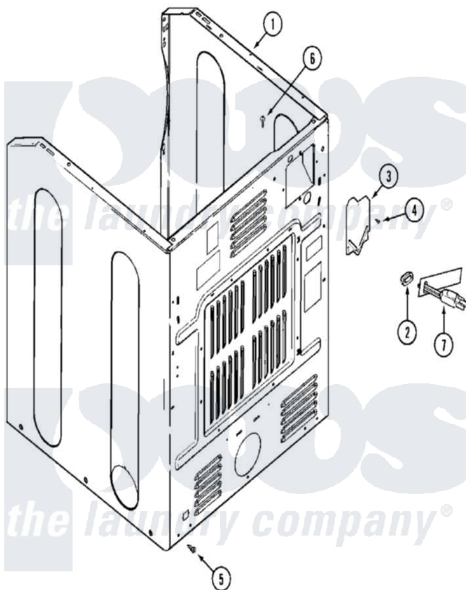
Maytag Commercial Maytag MLG23PDAGW Dryer Parts Parts Diagram 07 - CABINET-REAR Click on the part number to view part
