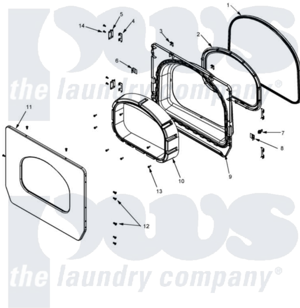
Maytag Commercial Maytag MLG23PDFXW Dryer Parts Parts Diagram 05 - DOOR Click on the part number to view part
