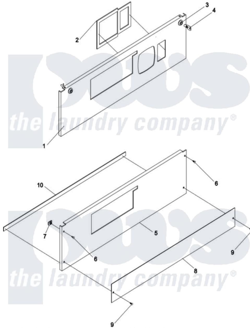
Maytag Commercial Maytag MLG31PCBWQ Dryer Parts Parts Diagram 01 - COIN CONTROL AND LINT DOOR ASSY
