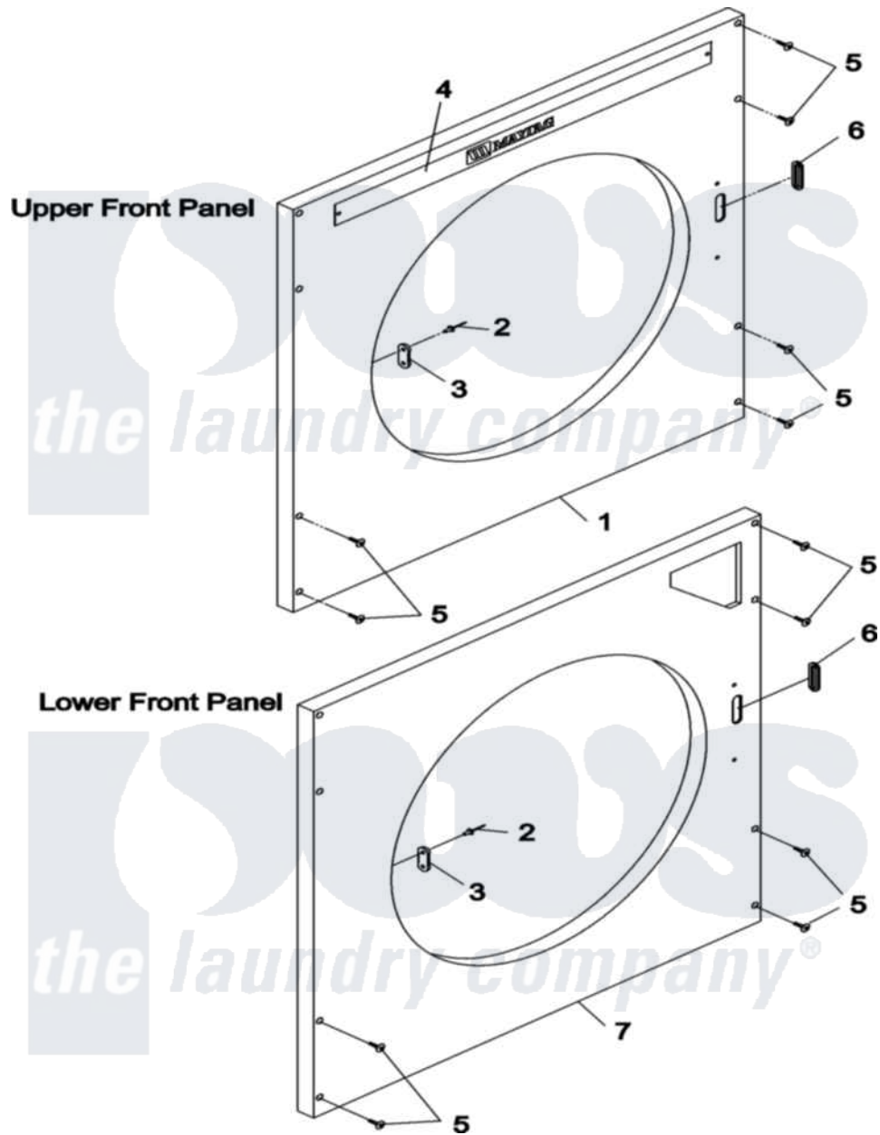
Maytag Commercial Maytag MLG31PCBWQ Dryer Parts Parts Diagram 06 - UPPER/LOWER FRONT PANEL Click on the part number to view part
