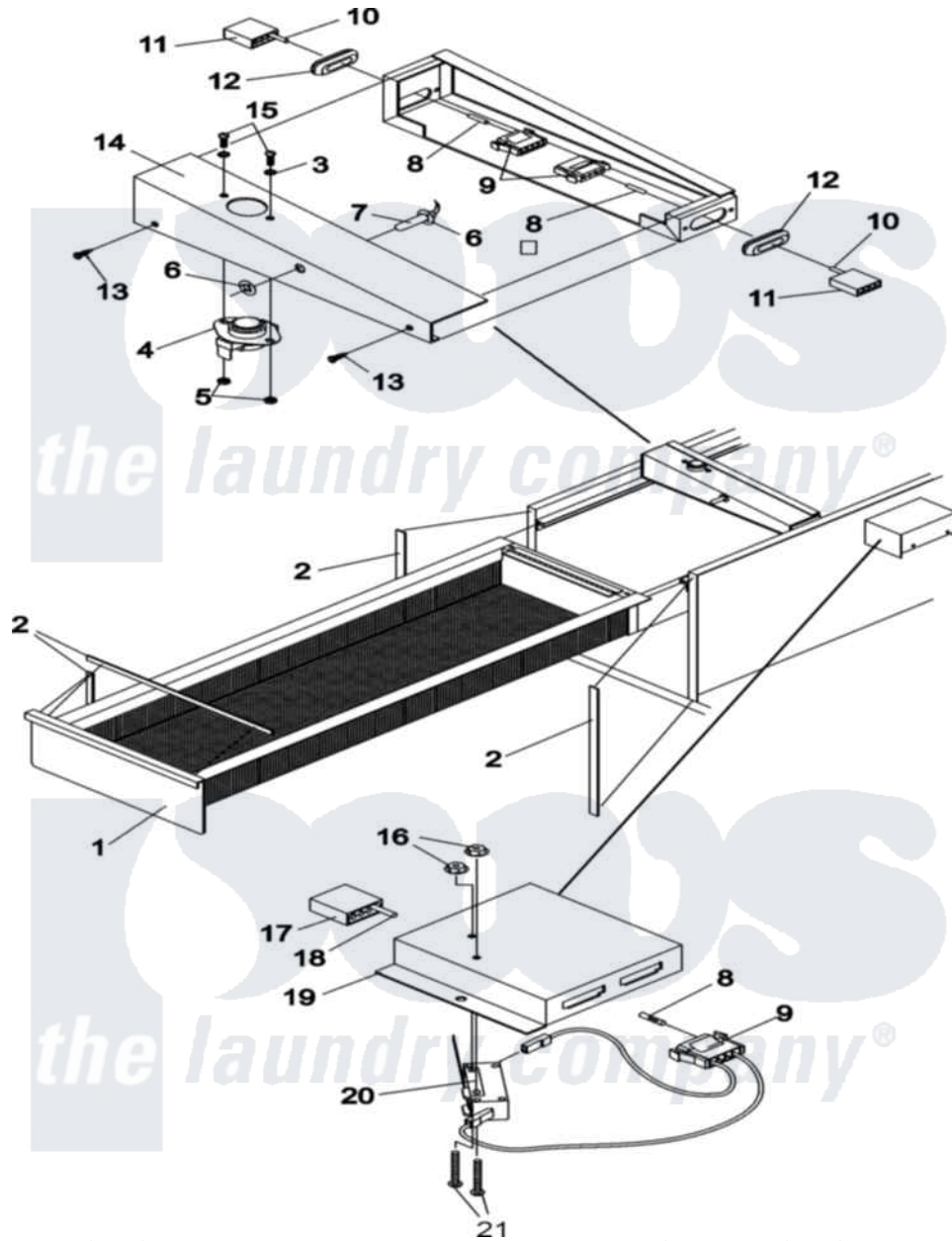
Maytag Commercial Maytag MLG31PCBWW Dryer Parts Parts Diagram 02 - LINT DRAWER W/TEMP AND SWITCH ASSY
