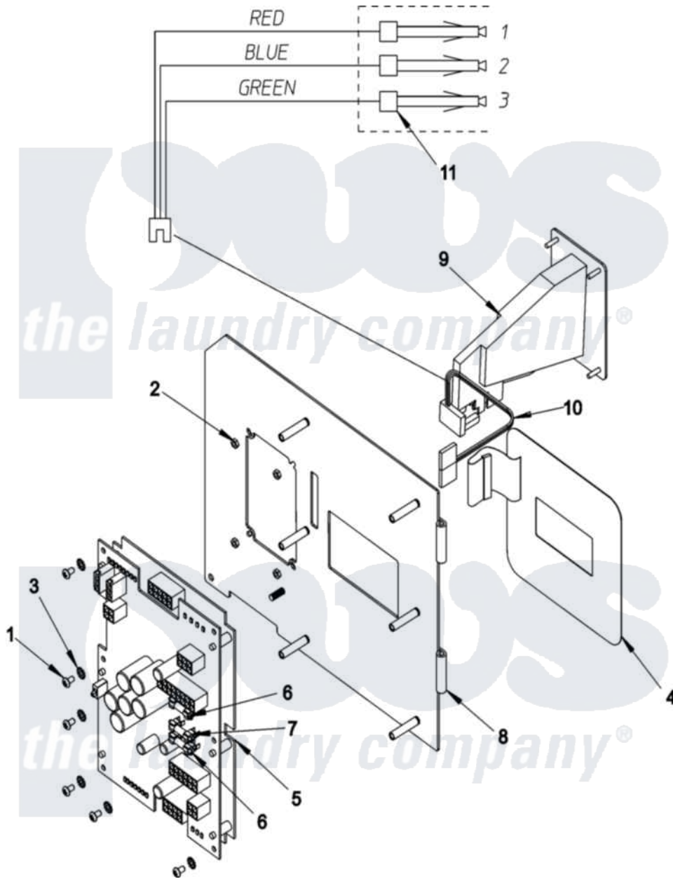
Maytag Commercial Maytag MLG31PCBWW Dryer Parts Parts Diagram 03 - DMC CONTROL PANEL ASSEMBLY
