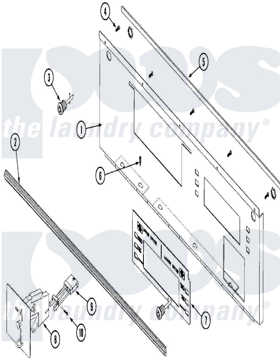
Maytag Commercial Maytag MLG32PDAWA Dryer Parts Parts Diagram 01 - CONTROL DOOR ASSEMBLY Click on the part number to view part
