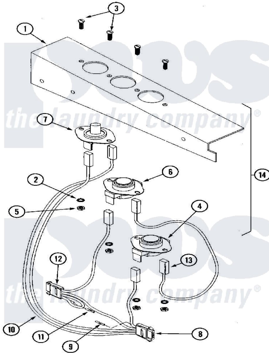
Maytag Commercial Maytag MLG32PDAWA Dryer Parts Parts Diagram 08 - TEMP. SENSOR BRKT. ASSEMBLY (MLG32PDAWx)
