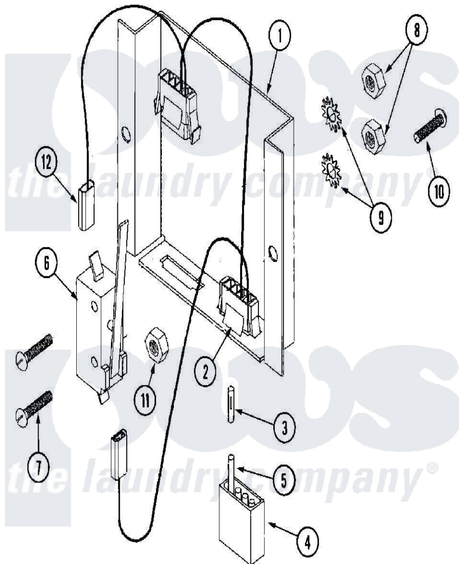
Maytag Commercial Maytag MLG32PDAWA Dryer Parts Parts Diagram 09 - LINT DRAWER SWITCH ASSEMBLY (MLG32PDAWx)
