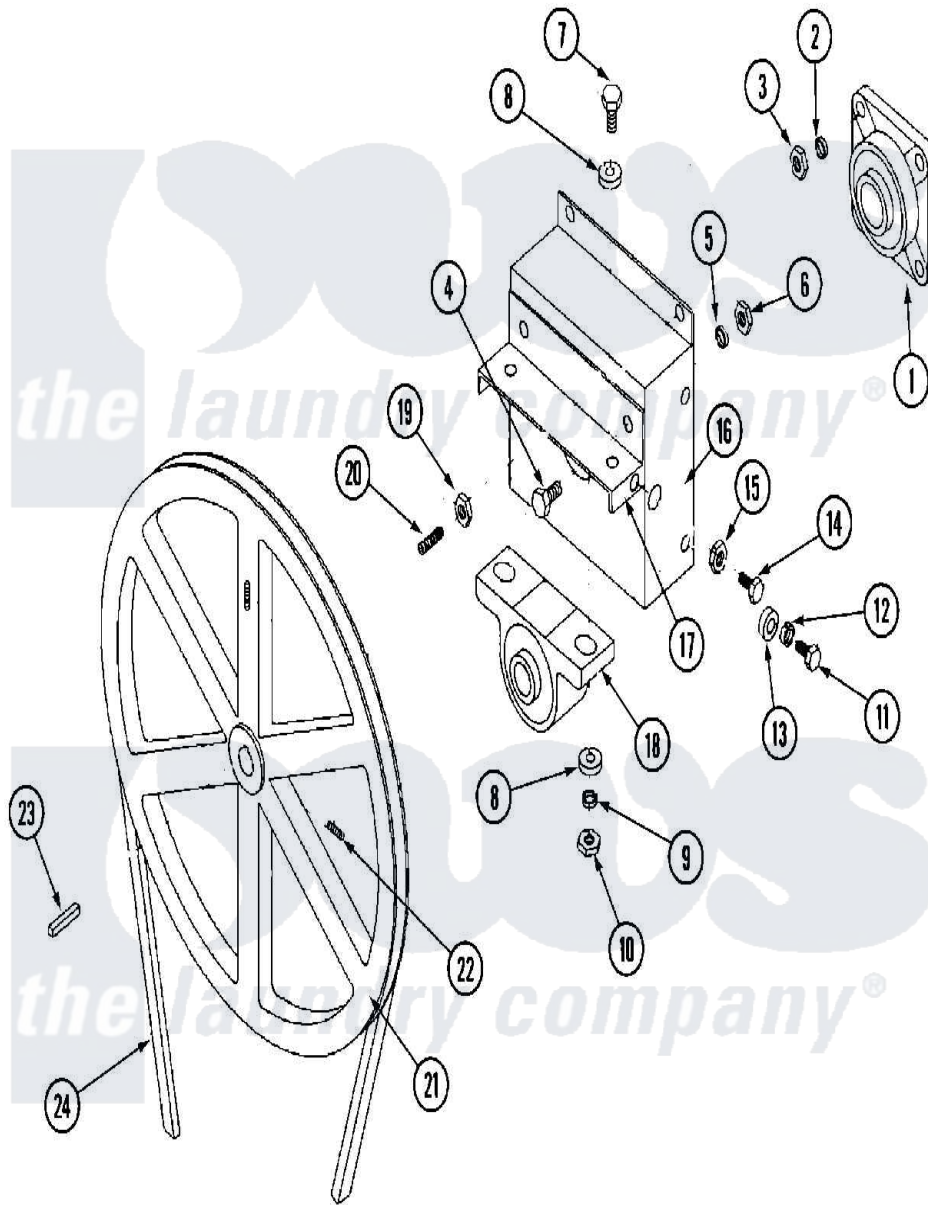
Maytag Commercial Maytag MLG32PDAWA Dryer Parts Parts Diagram 11 - TUMBLER BEARING ASSEMBLY (MLG32PDAWx)
