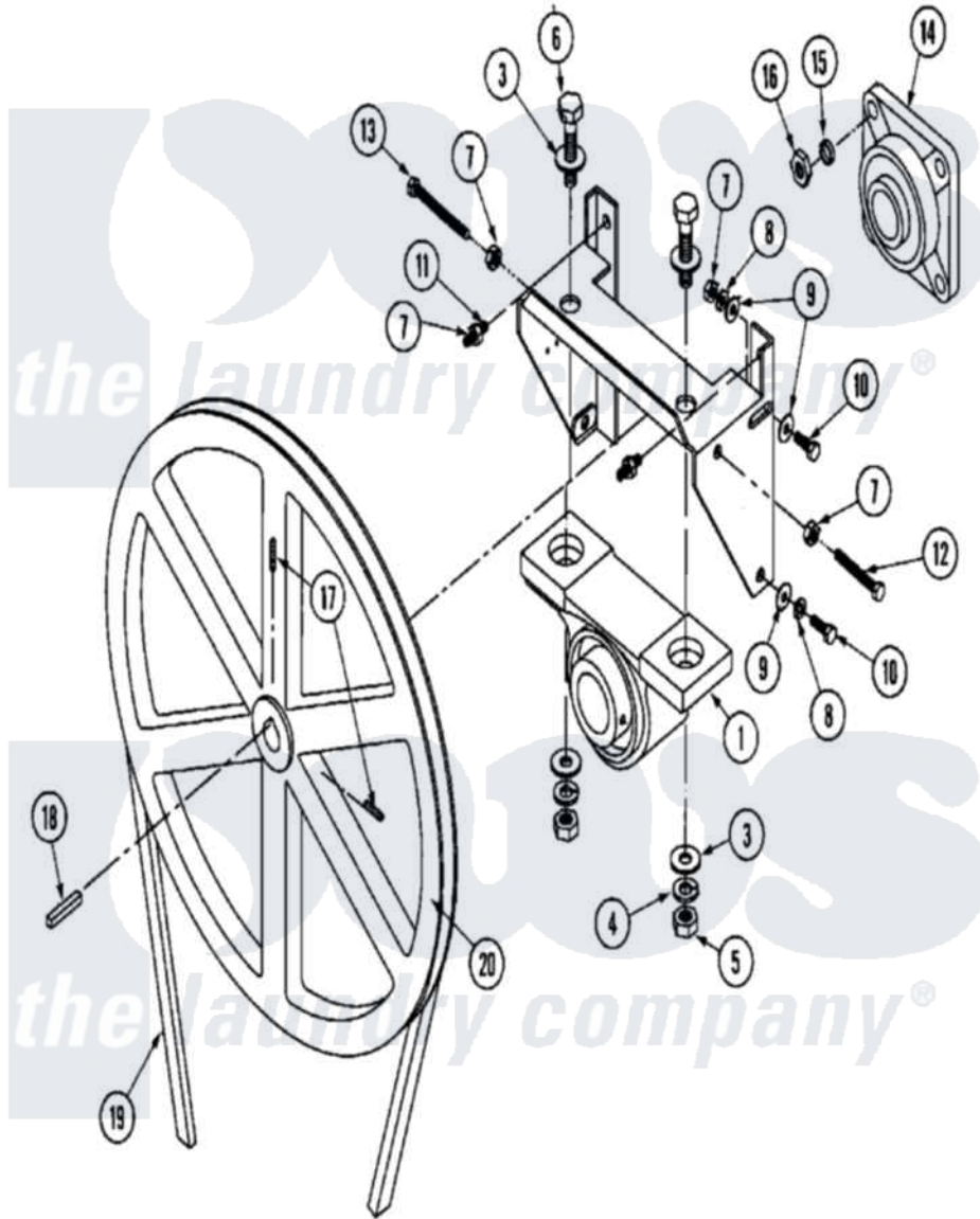
Maytag Commercial Maytag MLG32PDAWA Dryer Parts Parts Diagram 25 - TUMBLER BEARING ASSEMBLY (MLG32PDBWx)
