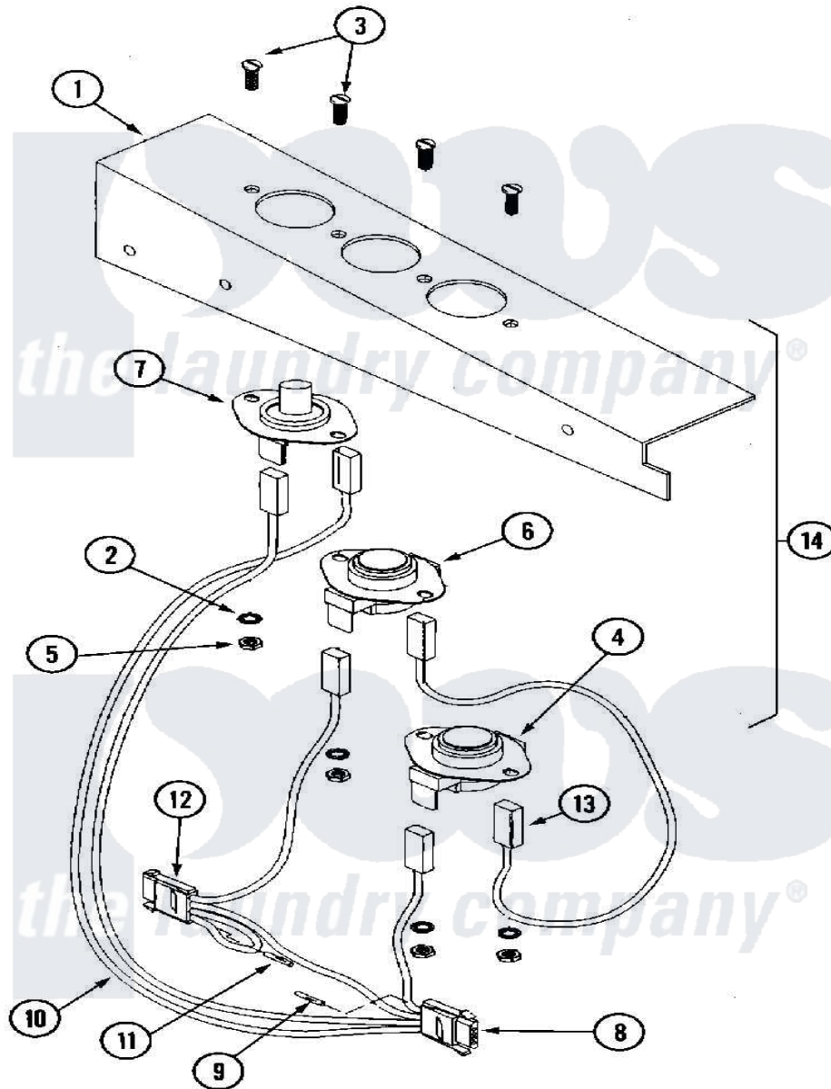
Maytag Commercial Maytag MLG32PDAWW Dryer Parts Parts Diagram 08 - TEMP. SENSOR BRKT. ASSEMBLY (MLG32PDAWx)
