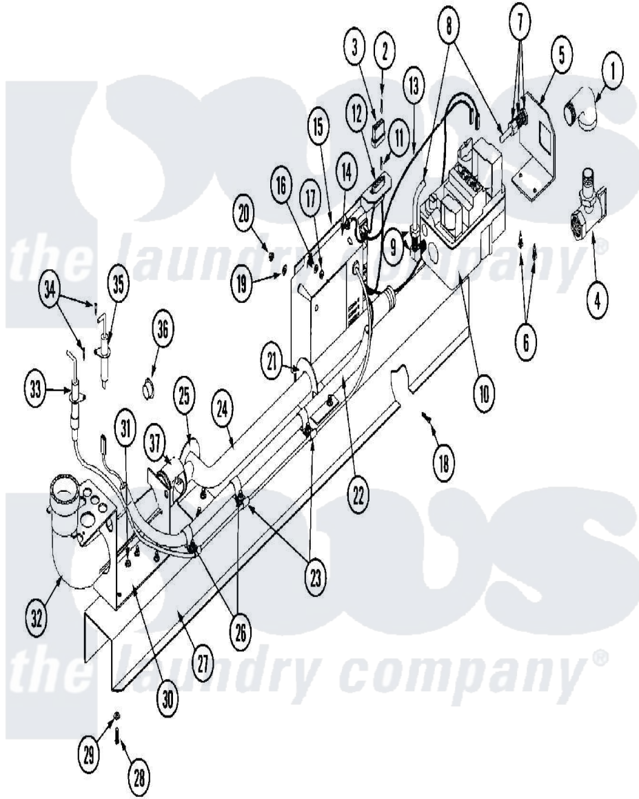
Maytag Commercial Maytag MLG32PDAWW Dryer Parts Parts Diagram 13 - GAS VALVE ASSEMBLY (PRIOR TO YW SERIALNo.)
