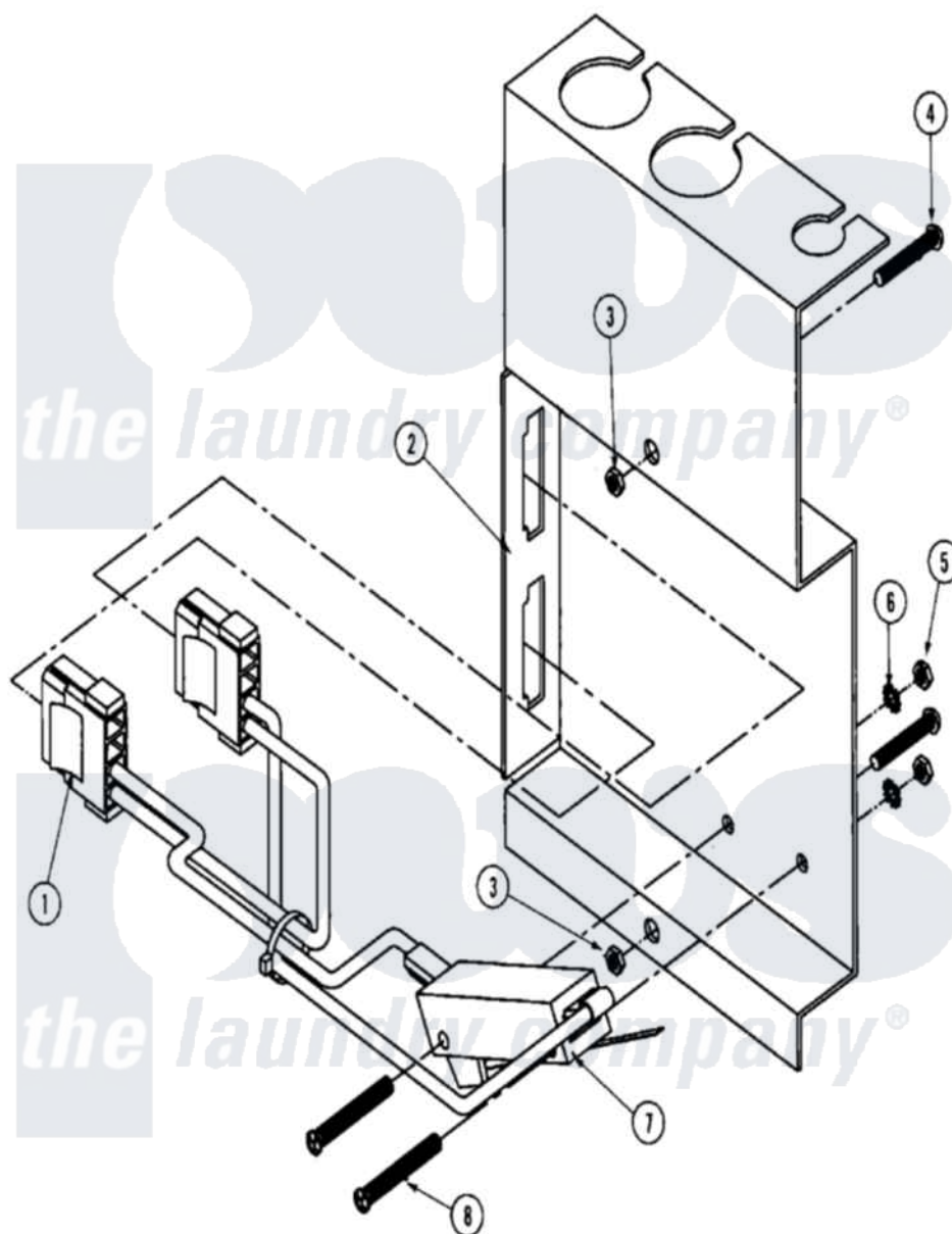
Maytag Commercial Maytag MLG32PDAWW Dryer Parts Parts Diagram 23 - LINT DRAWER SWITCH ASSEMBLY (MLG32PDBWx)
