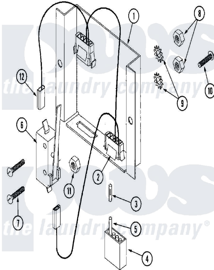
Maytag Commercial Maytag MLG32PDBWW Dryer Parts Parts Diagram 08 - LINT DRAWER SWITCH ASSEMBLY (MLG32PDAWx)
