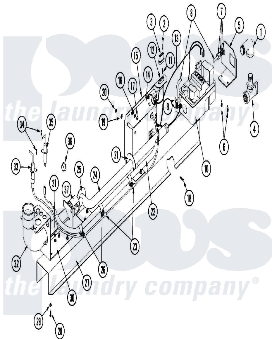
Maytag Commercial Maytag MLG32PDBWW Dryer Parts Parts Diagram 11 - GAS VALVE ASSEMBLY (PRIOR TO YW SERIALNo.)
