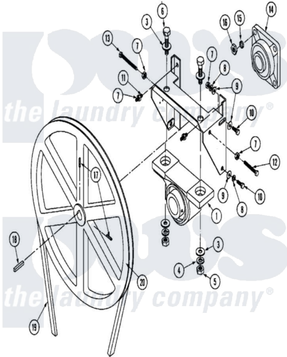
Maytag Commercial Maytag MLG32PDBWW Dryer Parts Parts Diagram 23 - TUMBLER BEARING ASSEMBLY (MLG32PDBWx)
