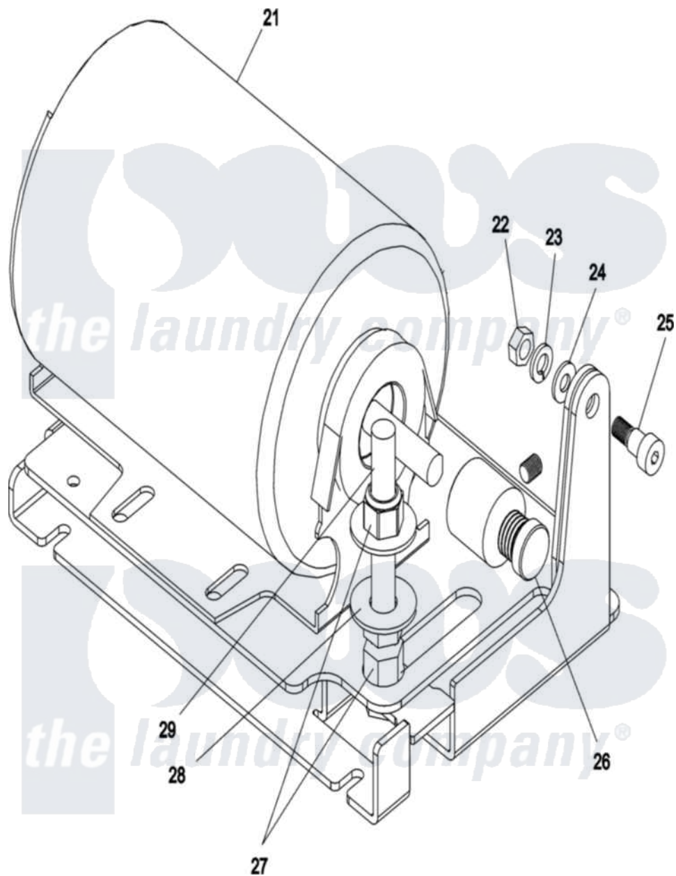
Maytag Commercial Maytag MLG33PDSWS Dryer Parts Parts Diagram 02 - MOTOR Click on the part number to view part
