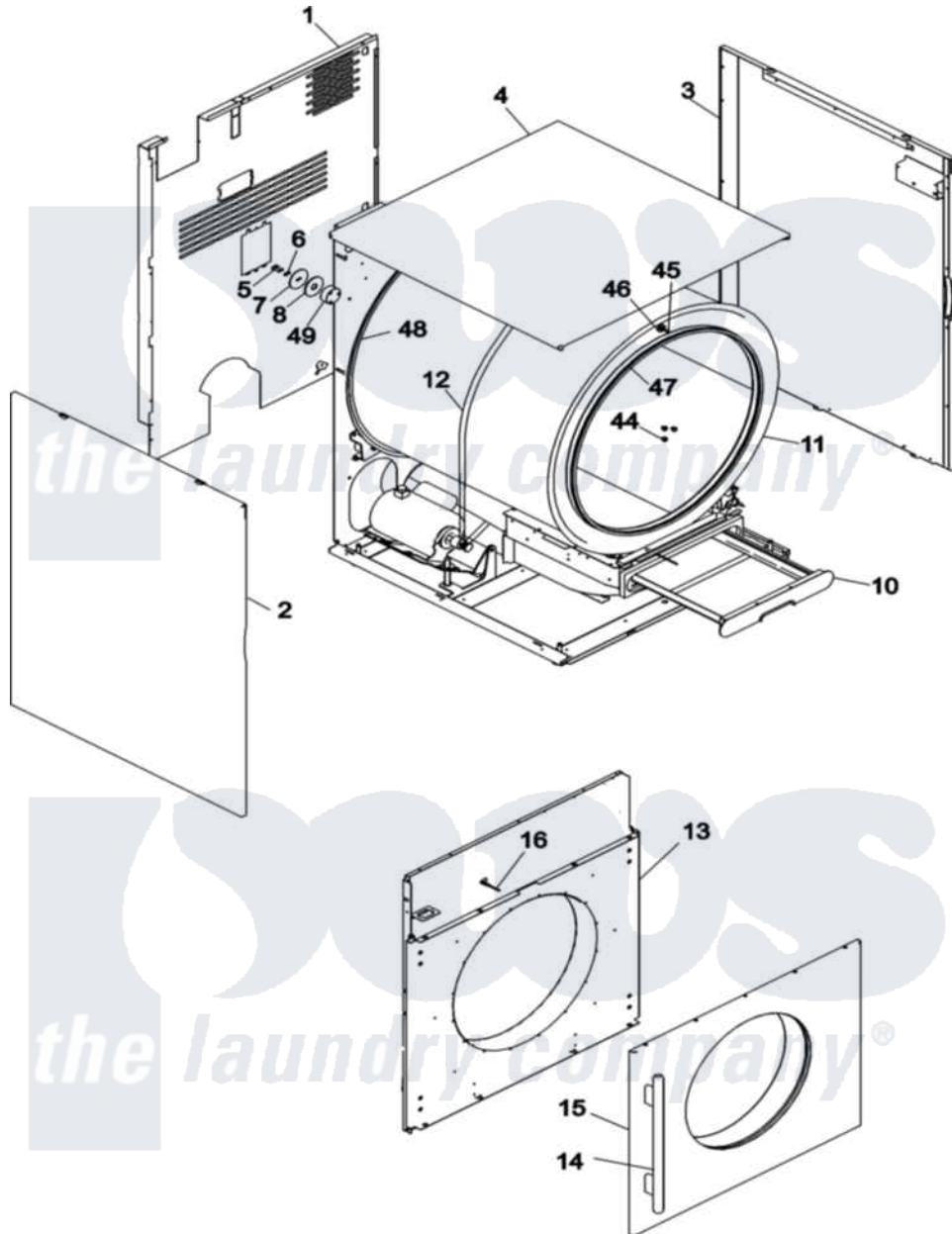
Maytag Commercial Maytag MLG33PDSWW Dryer Parts Parts Diagram 01 - CABINET Click on the part number to view part
