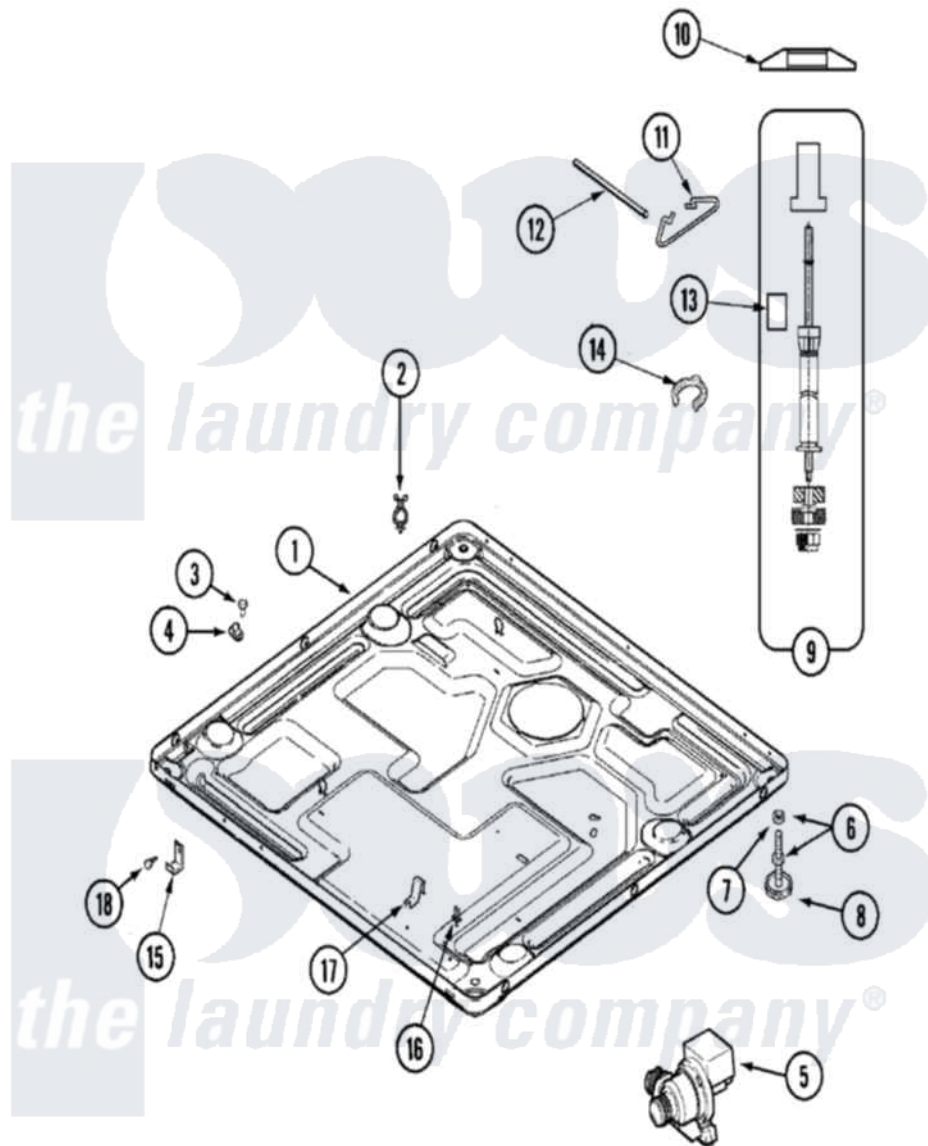
Maytag Commercial Maytag MUG2000AXW Stacked Washer and Dryer Parts Parts Diagram 01 - BASE (WASHER) Click on the part number to view part
