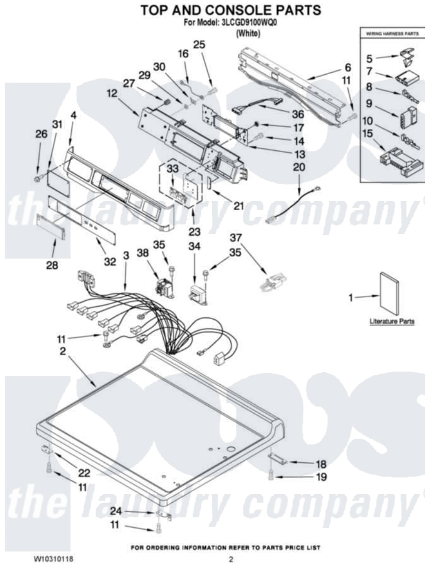
Whirlpool Commercial Whirlpool 3LCGD9100WQ0 Dryer Parts Parts Diagram 01 - TOP AND CONSOLE PARTS Click on the part number to view part
