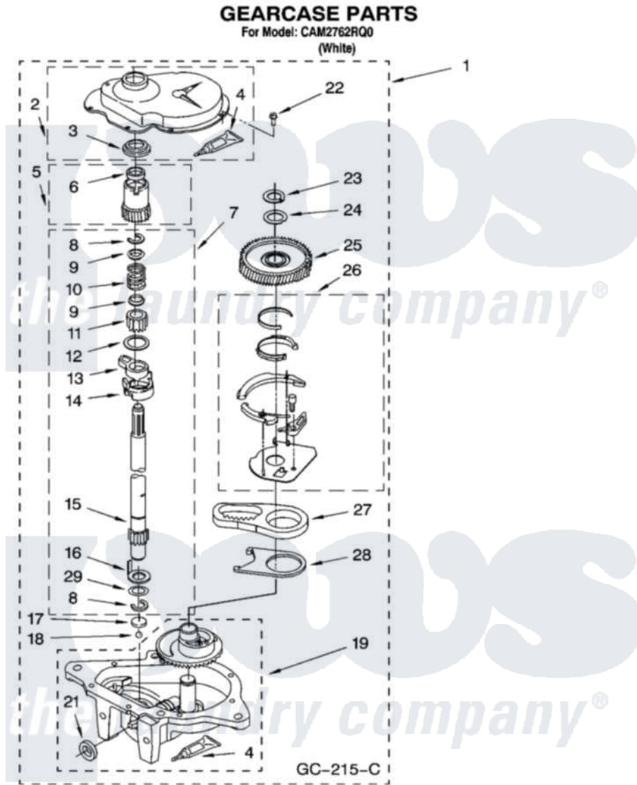
Whirlpool Commercial Whirlpool CAM2762RQ0 Washer Parts Parts Diagram 10 - GEARCASE PARTS Click on the part number to view part
