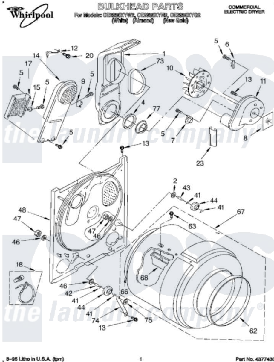
Whirlpool Commercial Whirlpool CE2950XYN2 Dryer Parts Parts Diagram 01 - SECTION Click on the part number to view part
