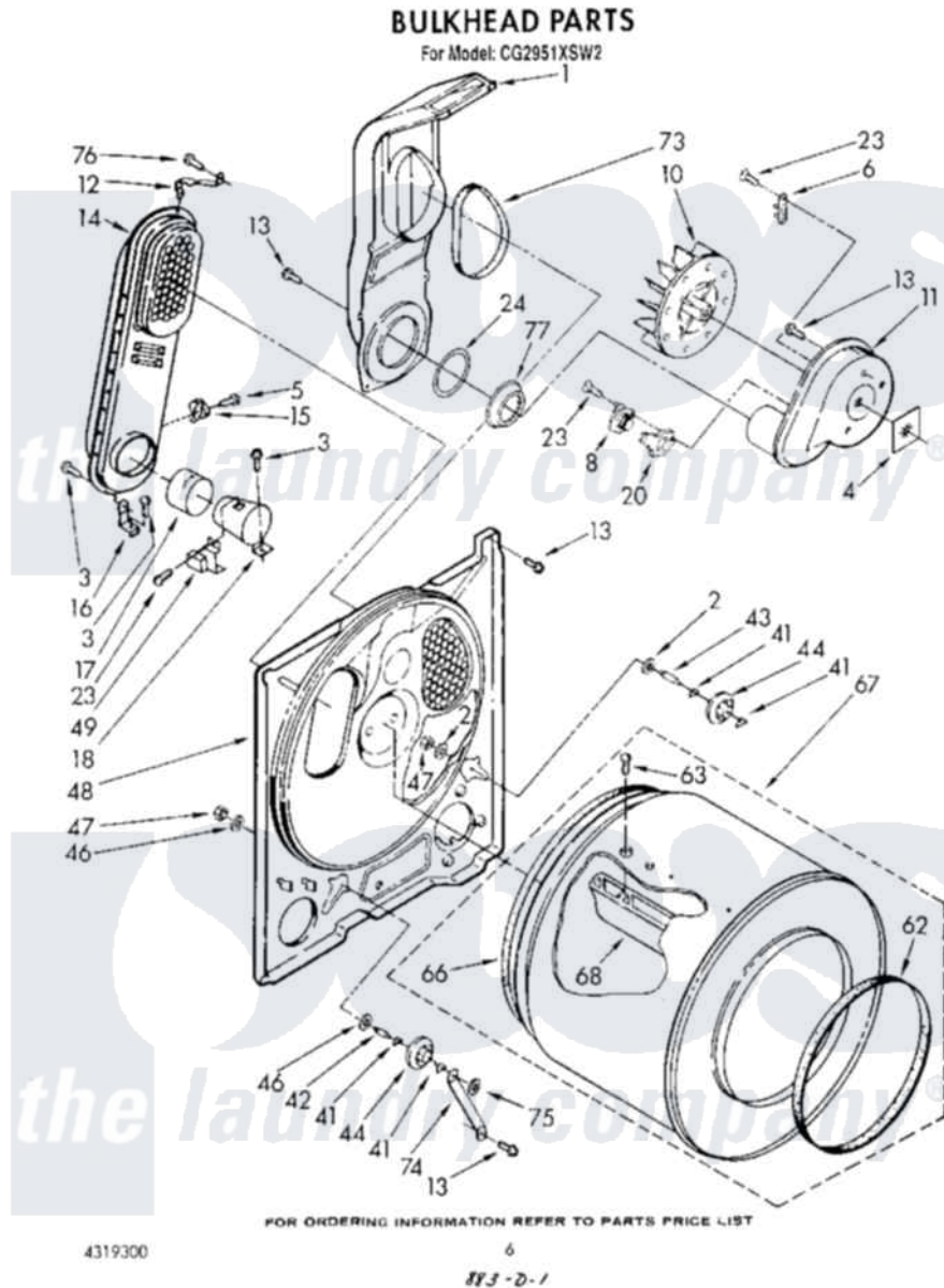
Whirlpool Commercial Whirlpool CG2951XSW2 Dryer Parts Diagram 04 - BULKHEAD , LIT/OPTIONAL Click on the part number to view part
