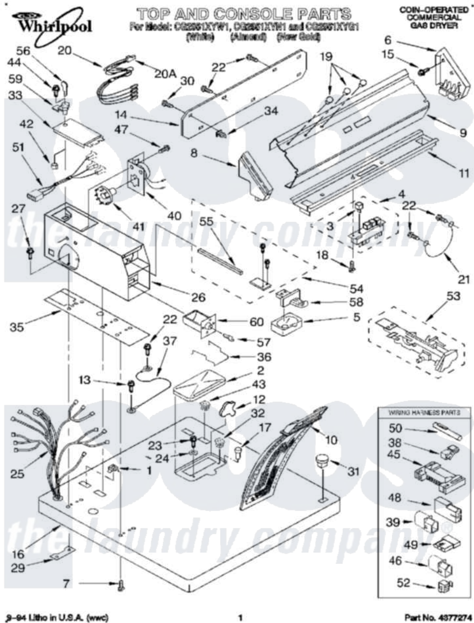
Whirlpool Commercial Whirlpool CG2951XYG1 Dryer Parts Parts Diagram 01 - TOP AND CONSOLE Click on the part number to view part
