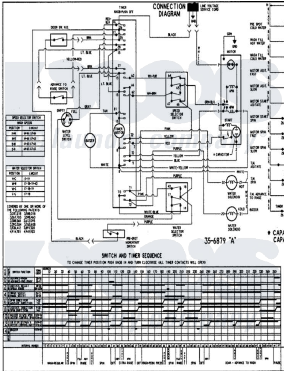
Admiral Residential Admiral AAV800AWW Washer Parts Parts Diagram 08 - WIRING INFORMATION
