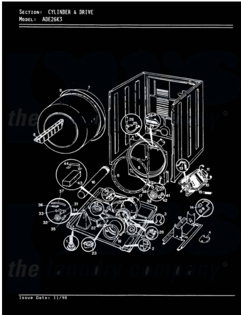
Admiral Residential Admiral ADE26K3A Dryer Parts Parts Diagram 02 - CYLINDER & DRIVE (REV. A-C) Click on the part number to view part
