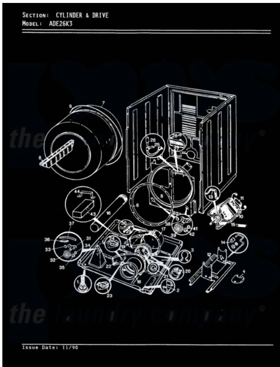
Admiral Residential Admiral ADE26K3W Dryer Parts Parts Diagram 02 - CYLINDER & DRIVE (REV. A-C) Click on the part number to view part
